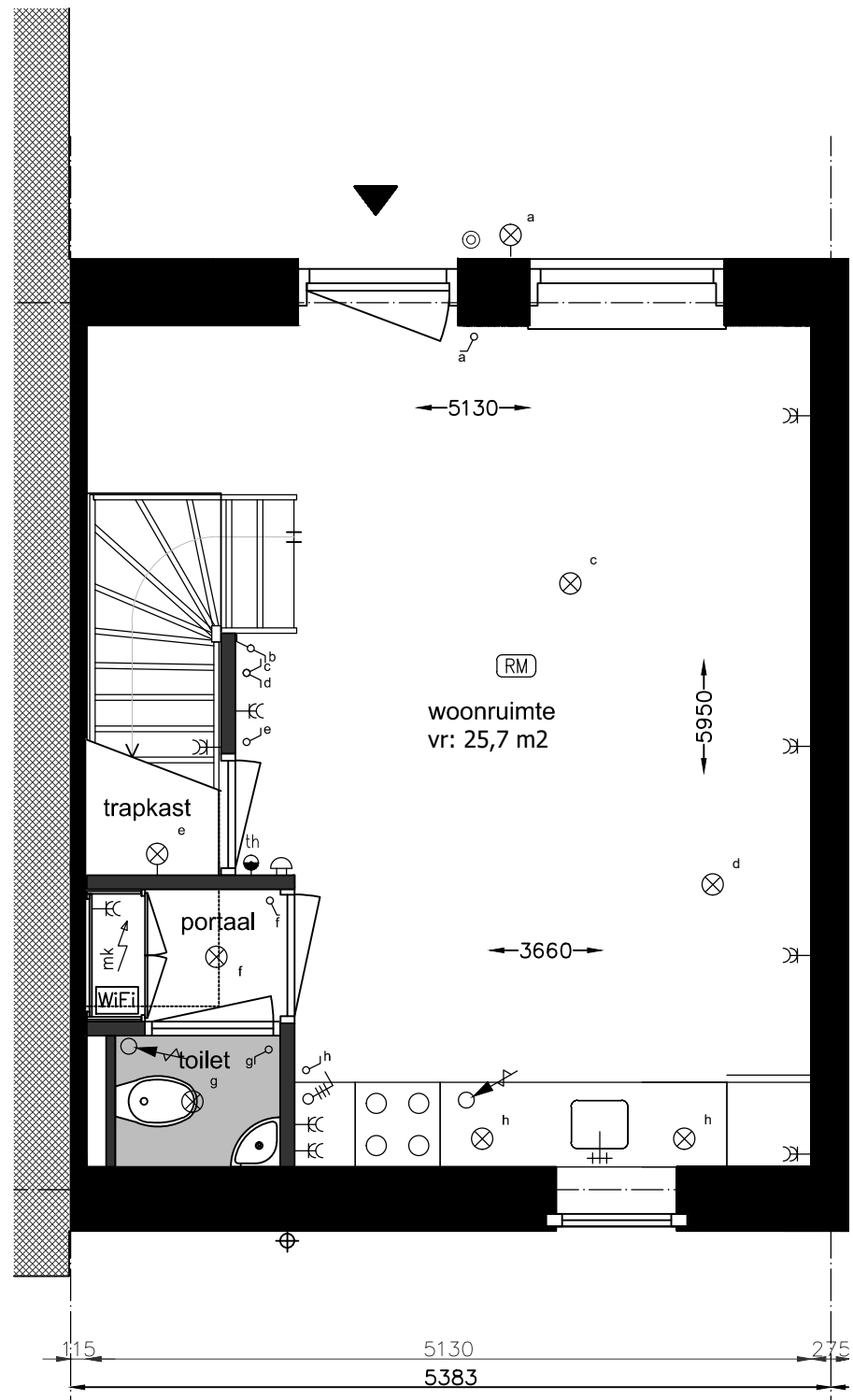
Begane Grond ↙ 1:50
