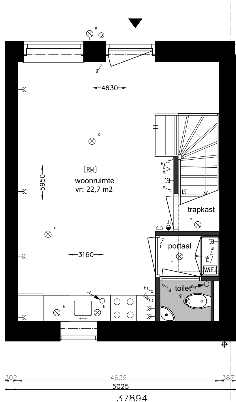
Begane Grond ↙ 1:50
