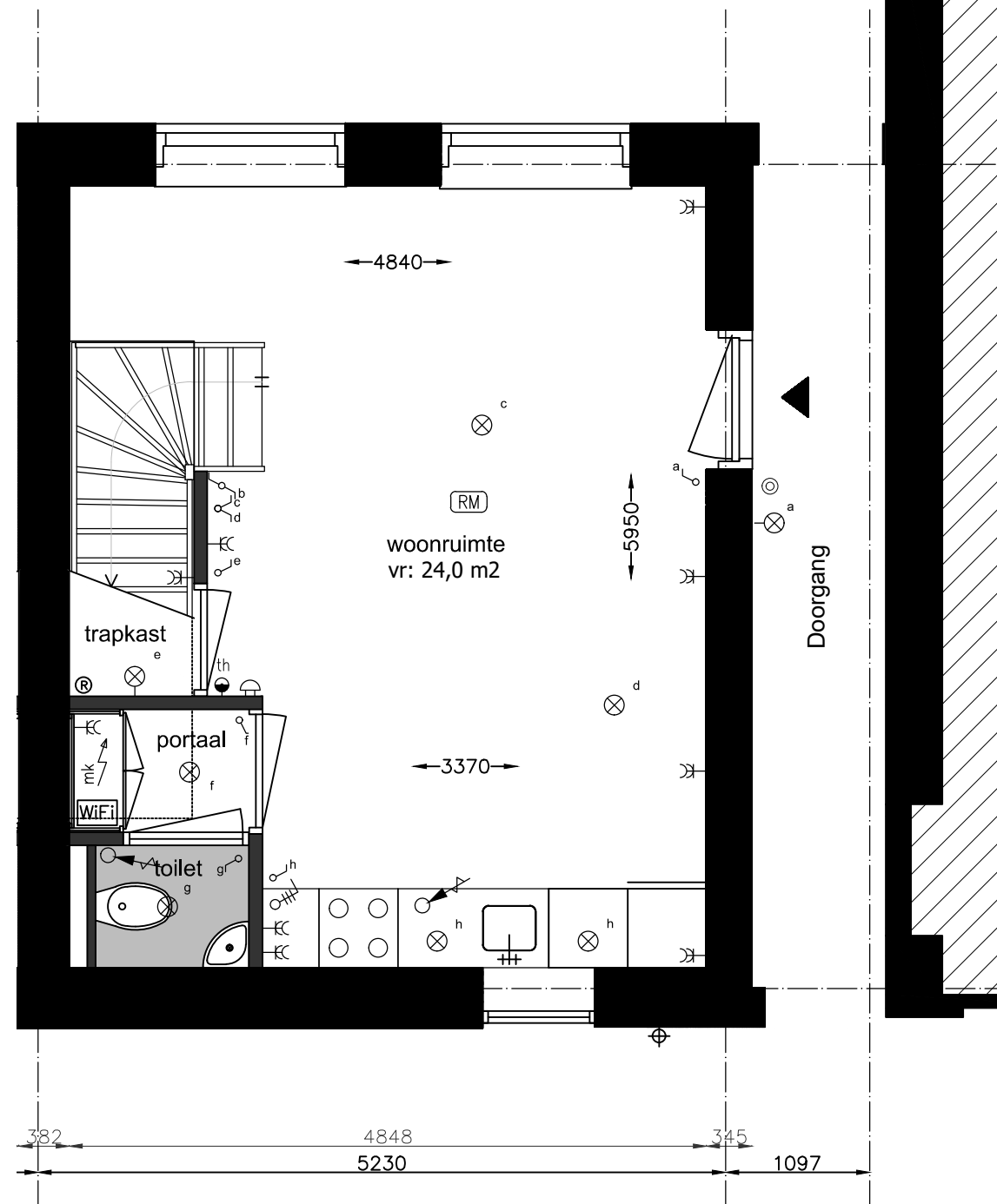
Begane Grond ↙ 1:50
